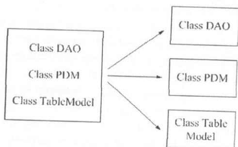
Figure 3. Splitting of Large Class
