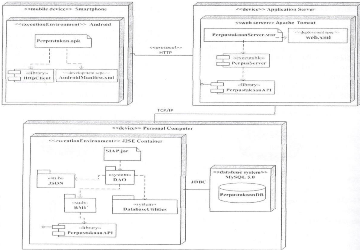
Figure 5. Deployment Diagram
