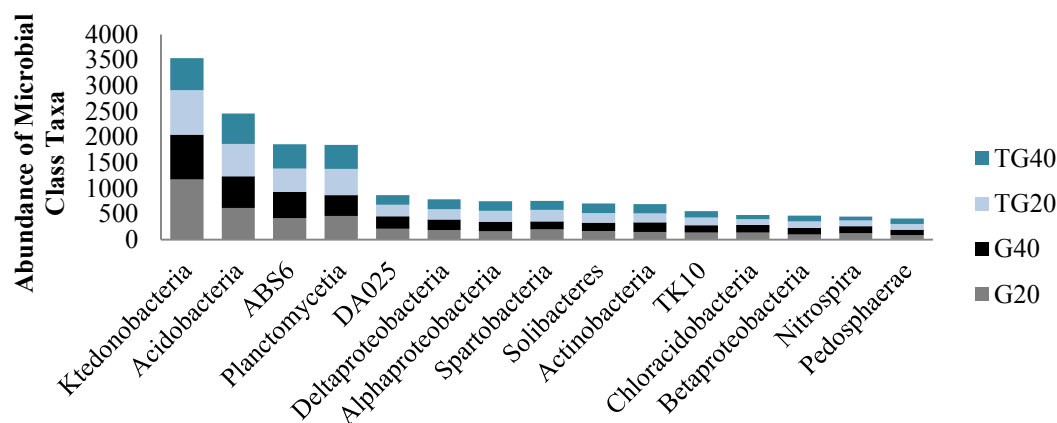
Figure 3. Abundance of top 15 classes taxa in G and TG soils with different soil depth.
