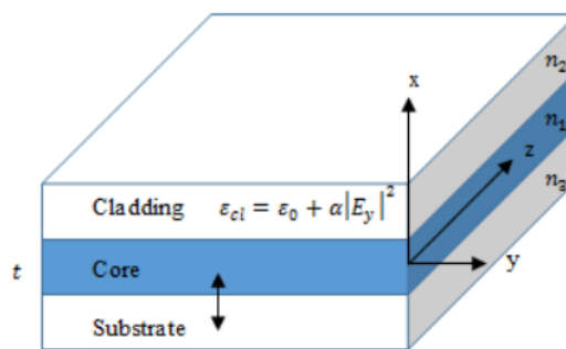
Figure 1. Asymmetric Waveguide
