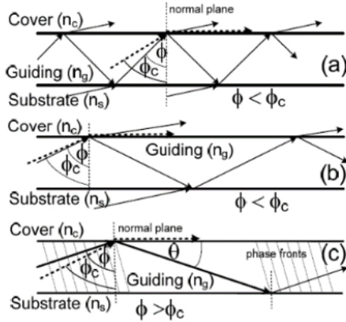
Figure 2. The ray picture of mode on an-symmetric step index slab waveguide [1]
