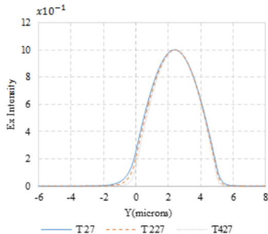
Figure 4. The Transverse Electric Mode Pattern
