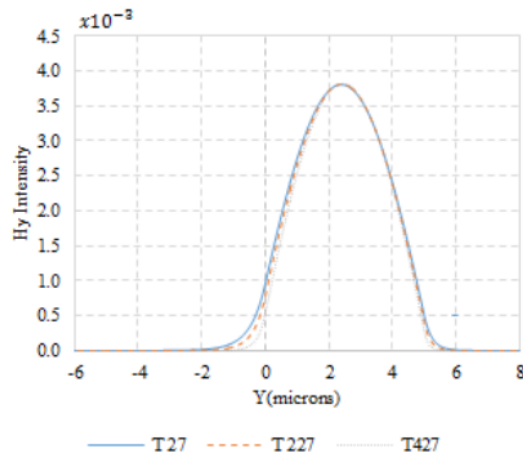
Figure 5. The Transverse Magnetic Mode Pattern
