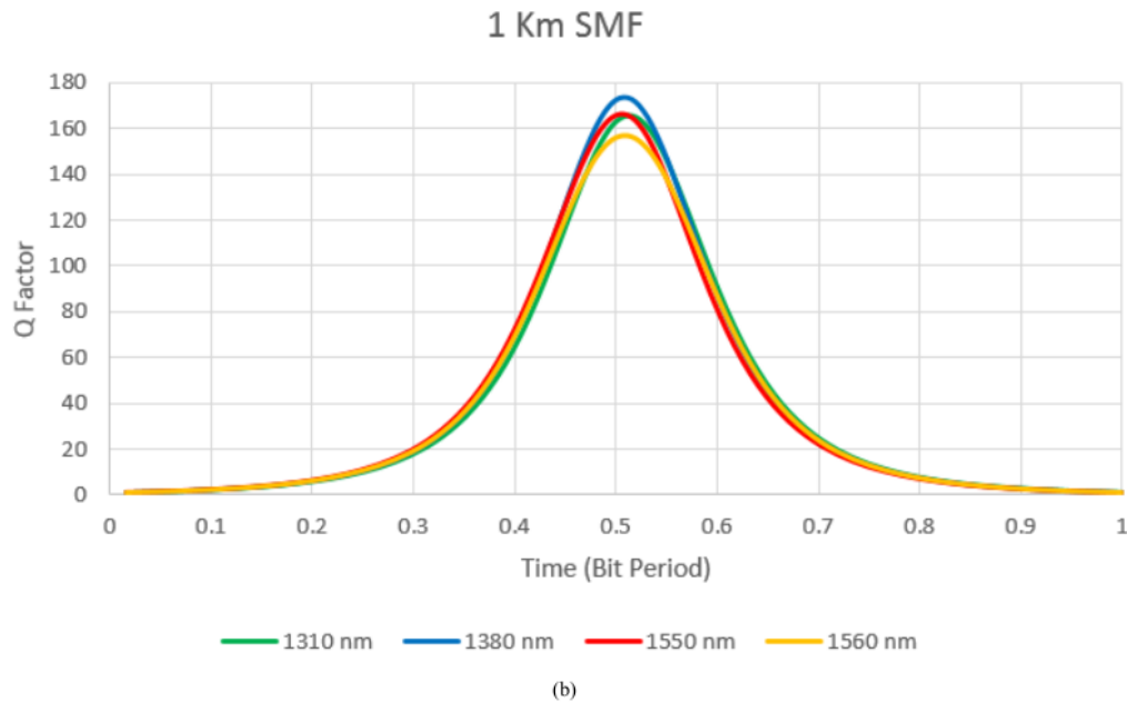
Figure 3. (a) Graph Q Factor FSO with Wavelength 1310 nm, 1380 nm, 1550 nm, and 1560 nm at 1 km. (b) Graph Q Factor SMF with Wavelength 1310 nm, 1380 nm, 1550 nm, and 1560 nm at 1 km
