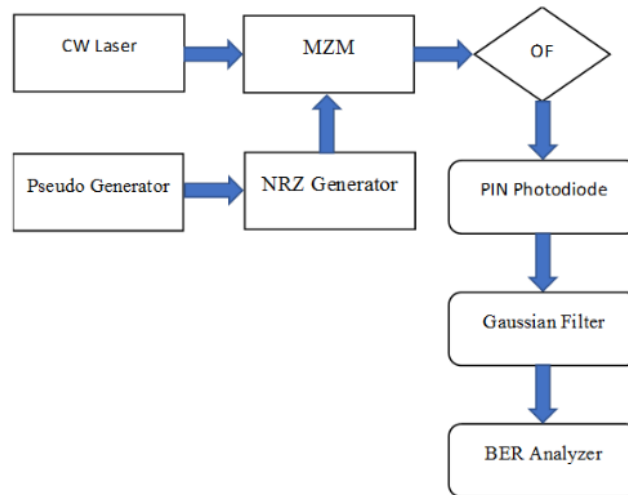
Figure 1. Design Optical Communication System
