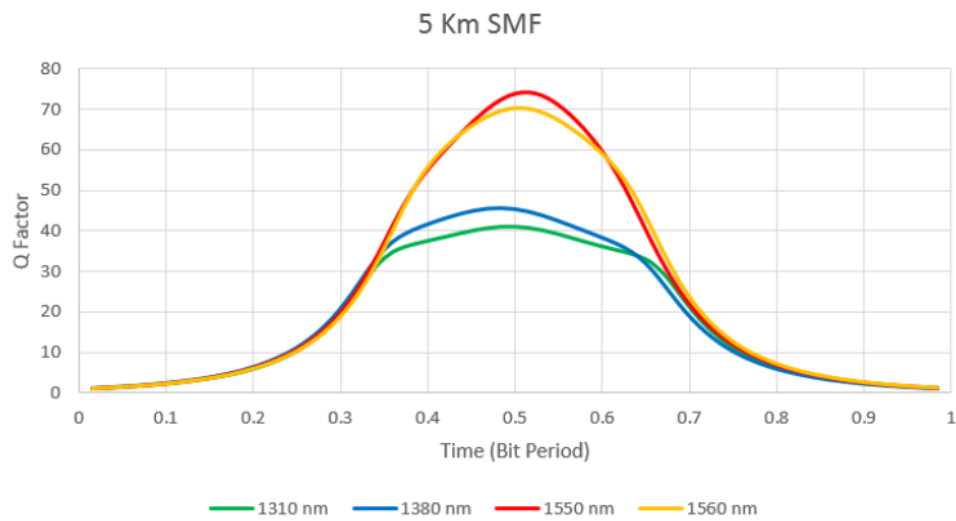
Figure 5. (a) Graph Q Factor FSO with Wavelength 1310 nm, 1380 nm, 1550 nm, and 1560 nm at 5 km (b) Graph Q Factor SMF with Wavelength 1310 nm, 1380 nm, 1550 nm, and 1560 nm at 5 km
