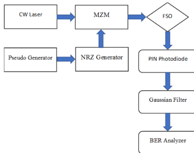
Figure 2. Design 3.2. Free Space Optics (FSO)
