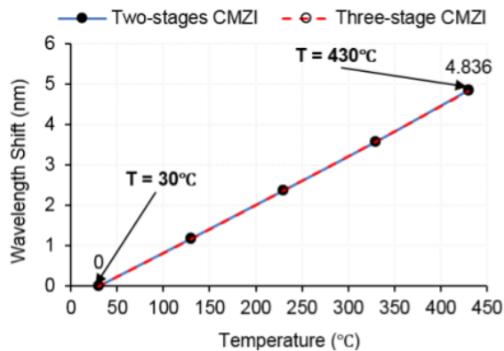
Figure 9. Wavelength shift as a function of temperatures
