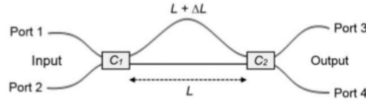
Figure 2. Two couplers MZI diagrams (single MZI)
