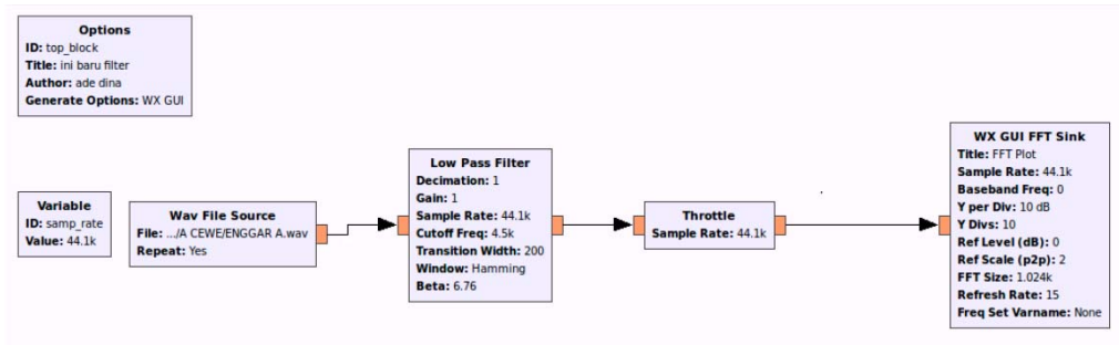
Figure 7 GRC block on GNU Radio for audio processing for gender identification.
