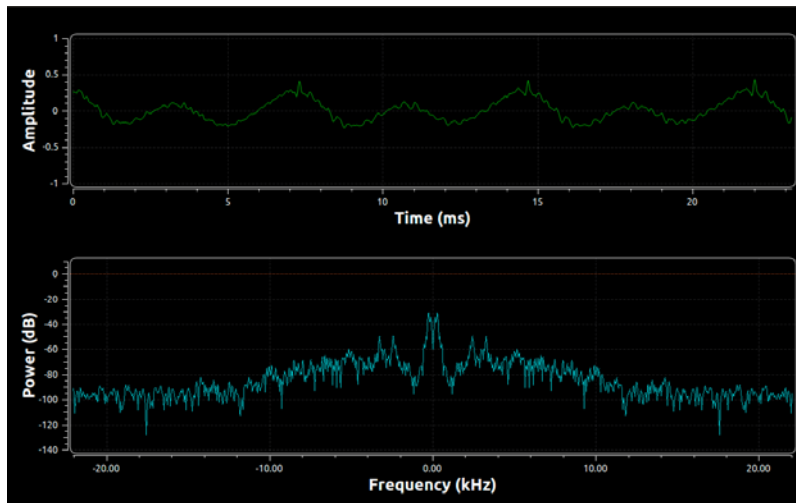
Figure 3 Output signal using sampling rate of 44.1 kHz, in Time Sink and Frequency Sink.
