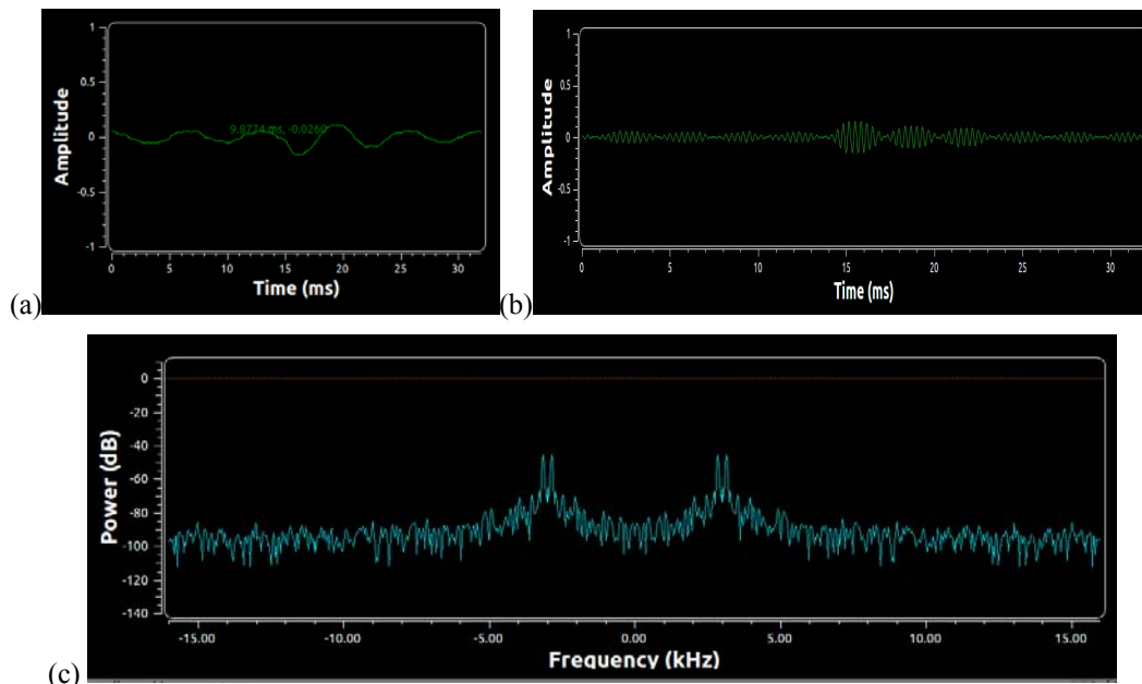
Figure 5 (a) Input audio (guitar instrument), (b) AM modulated signal, and (c) Frequency spectrum of modulated signal.
