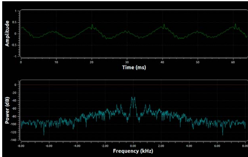
Figure 2 Output signal using sampling rate of 16 kHz, in Time Sink and Frequency Sink.
