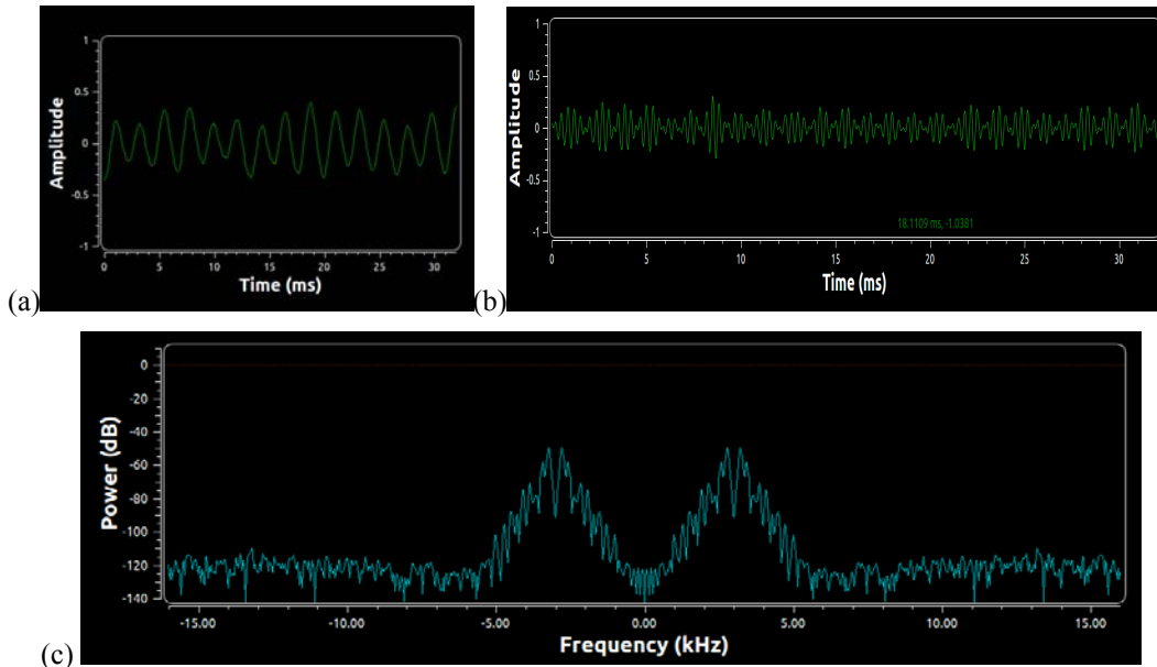
Figure 6 (a) Input audio (piano instrument), (b) AM modulated signal, and (c) Frequency spectrum of modulated signal.
