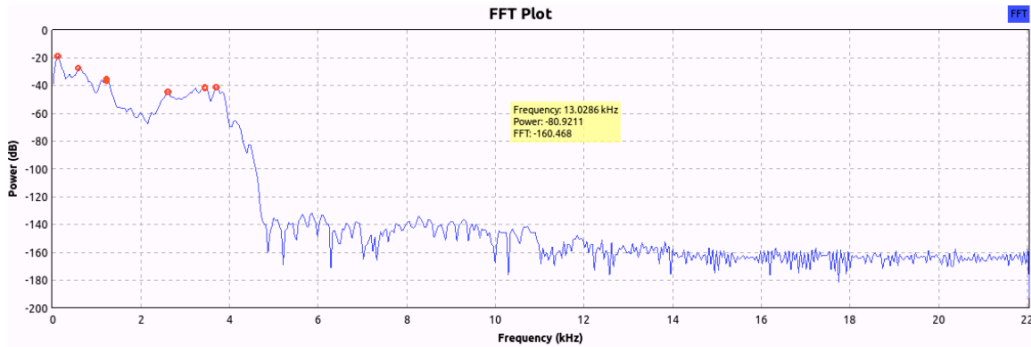
Figure 8 The example of frequency spectrum of male audio.
