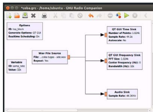
Figure 1. GRC block on GNU Radio for sampling rate adjustment for audio processing.
