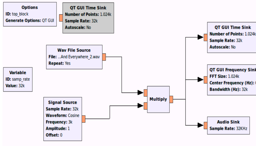
Figure 4 GRC block on GNU Radio for DSB-AM modulation technique.
