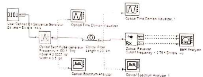
Fig. 3 Design Fiber with soliton parameters [1].
