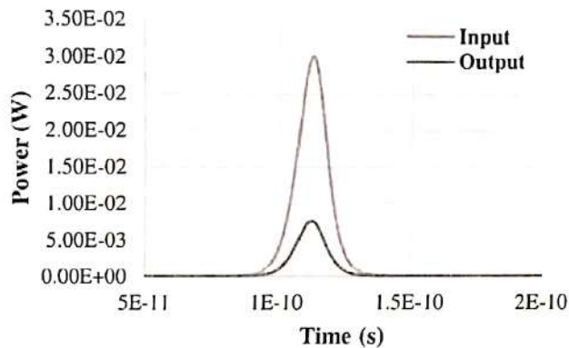
Fig. 5 Input and output of Fiber with-soliton parameter (using secant hyperbolic pulse)
