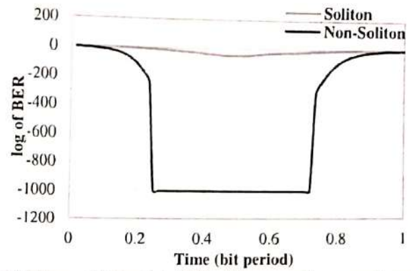
Fig. 6 Minimum Bit Error Rate (BER) of fiber non-soliton parameter and fiber with soliton parameter.
