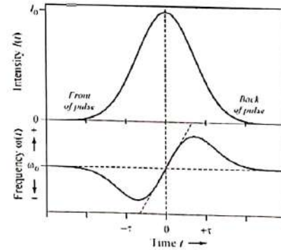
Fig. 1 Spectral broadening of a pulse due to SPM. [6]
