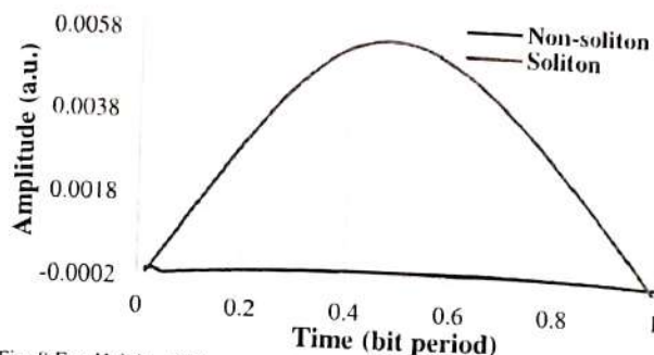
Fig. 8 Eye Height of fiber non-soliton parameter and fiber with soliton parameter.
