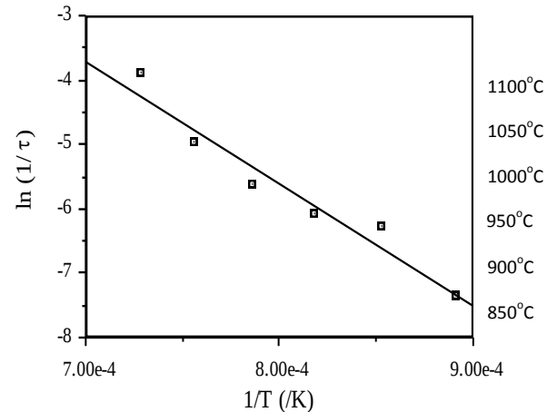
Figure 6. Variation of \ln(1/\tau) with 1/T
