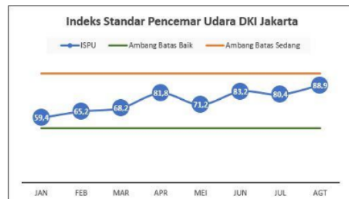
Fig. 1. Air pollution standard index DKI Jakarta 2019
