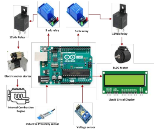
Fig. 9. Block diagram
