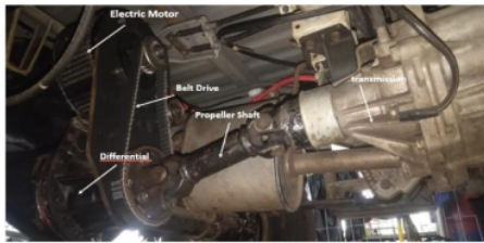
Fig. 3. Belt drive system
