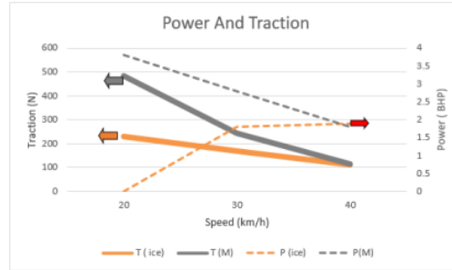
Fig. 8. Comparison of electric motor with ICE in 4th gear
