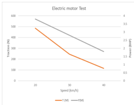
Fig. 6. Electric motor test
