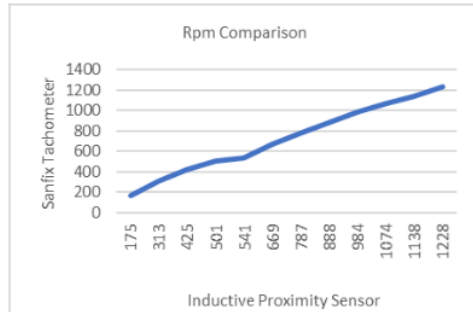
Fig. 10. Rpm comparison
